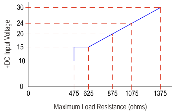
Figure 5 Maximum Load Resistance - Current Output
