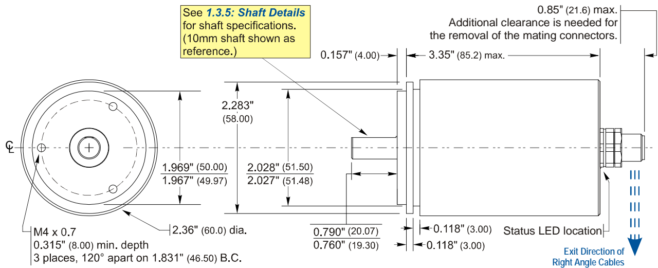
Figure 1.3 Servo Mount, End Connector Outline Drawing
