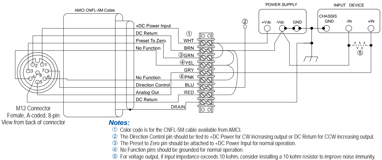
Figure 2.2 Sample Wiring Diagram
