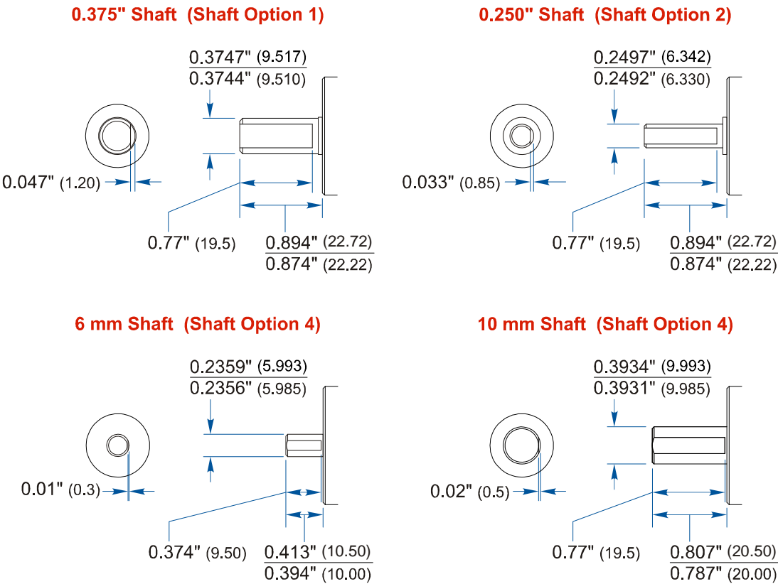
Figure 1.5 Shaft Details
