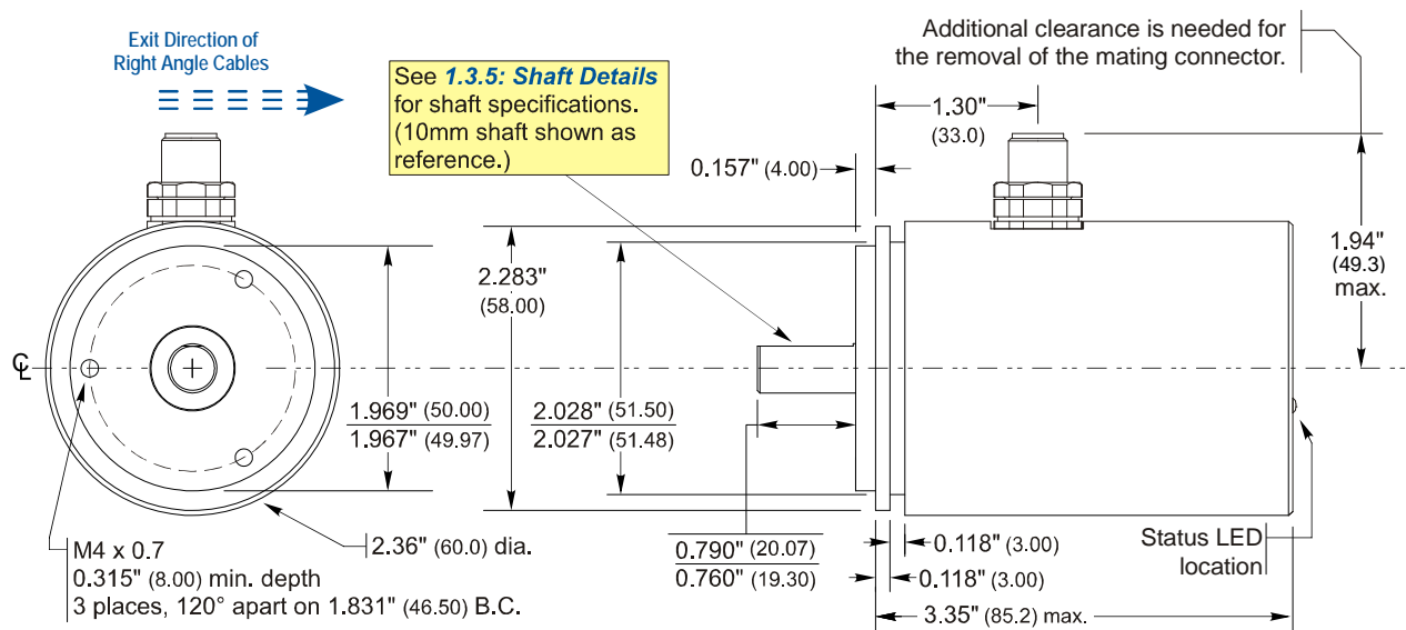
Figure 1.4 Servo Mount, Side Connector Outline Drawing
