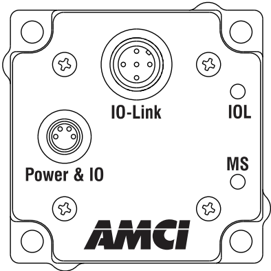
Figure R1.5 Rear Cover Status LED's
