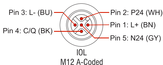
Figure R1.8 IO-Link Connector Pinout
