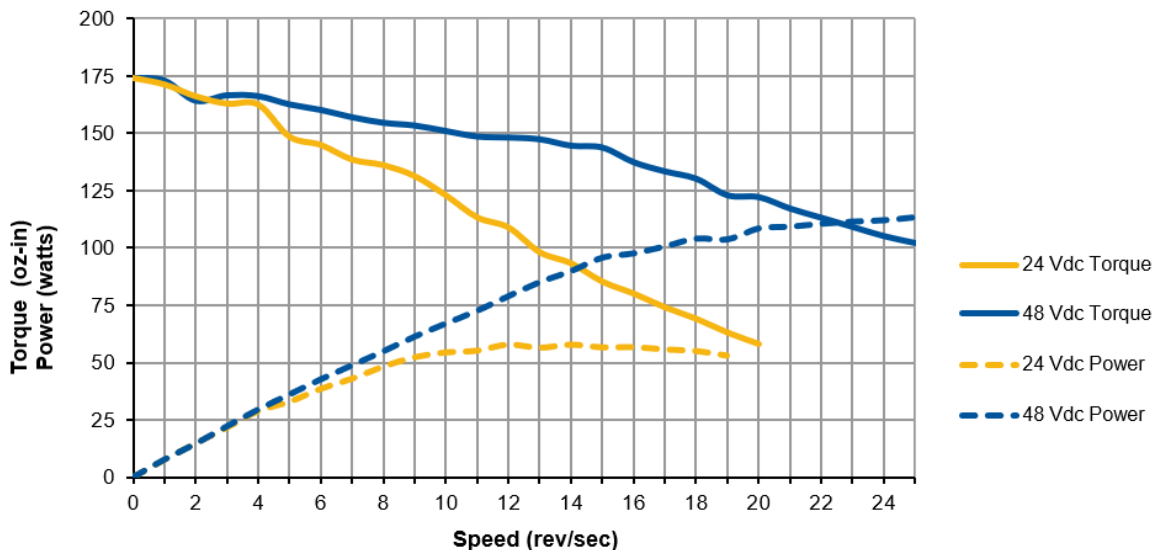
Figure R1.3 SMD23L-150 Torque and Power Curves
