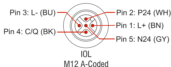
Figure T1.7 M12 IO-Link Connector Pinout
