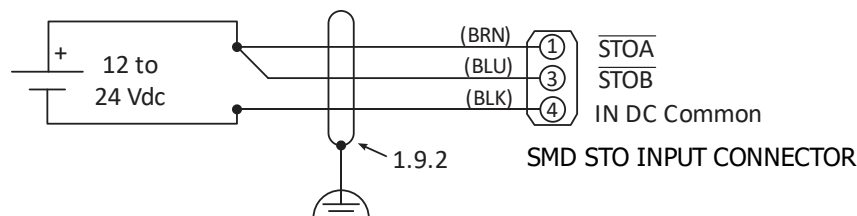
Figure T1.6 STO Input Connections
