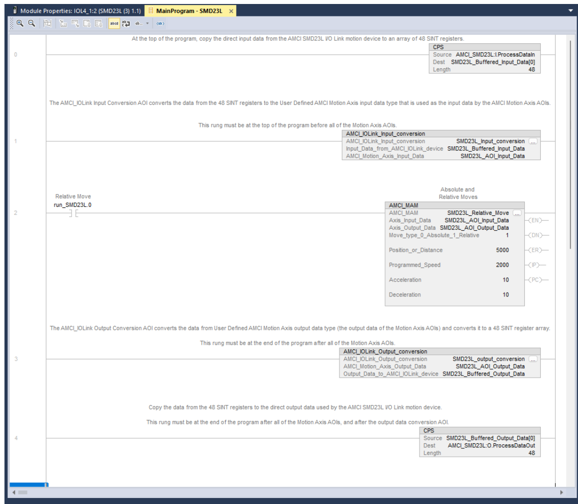
Figure T3.4 Sample Ladder Logic
