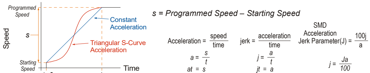
Figure R3.2 Move Profile Example
