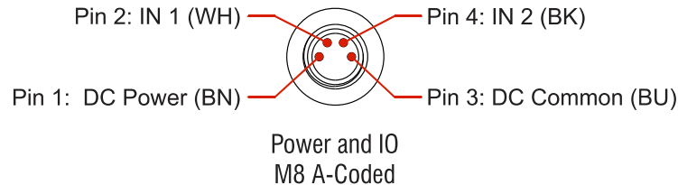
Figure R1.6 M8 Input Connector
