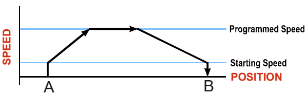
Figure R2.6 Absolute Move
