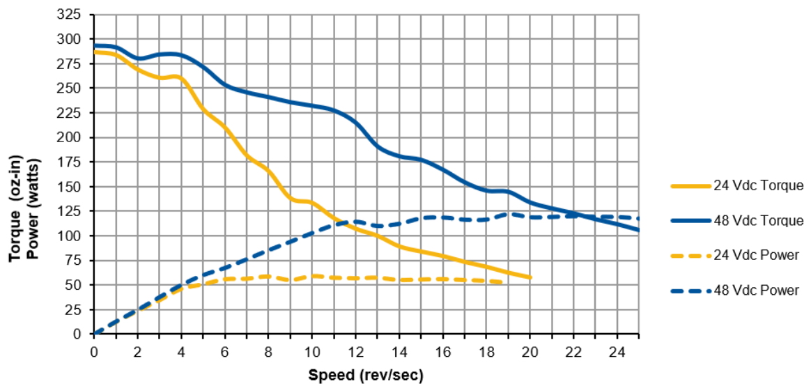
Figure R1.4 SMD23L-280 Torque and Power Curves
