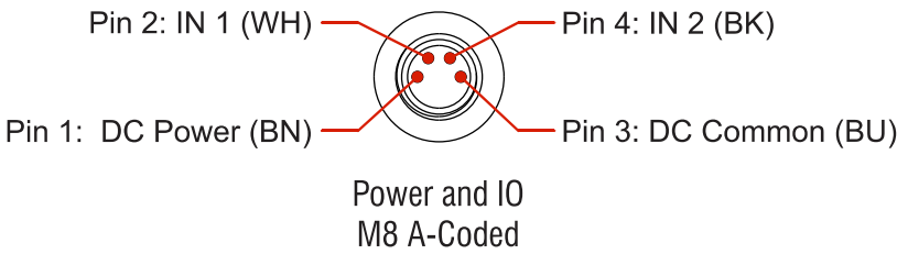
Figure T1.2 Power and Input Connector
