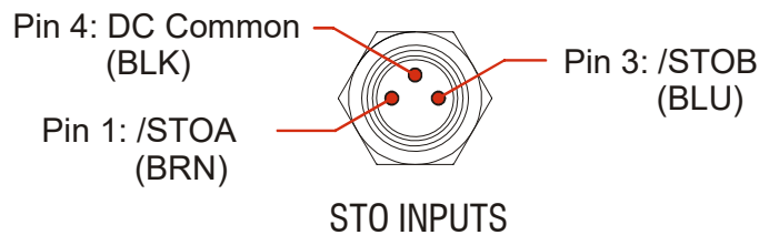
Figure T1.5 STO Input Wiring
