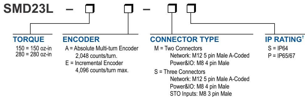
Figure R1.2 Part Numbering System
