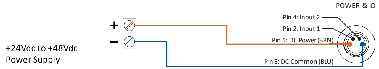
Figure T1.3 SMD23L Power Wiring
