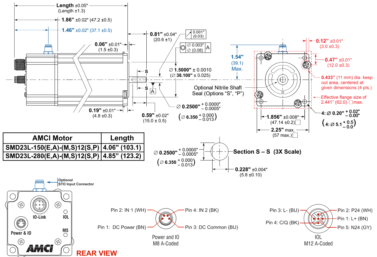
Figure T1.1 SMD23L-80 Outline Drawing
