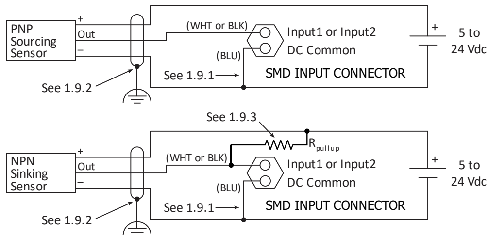
Figure T1.4 Input Wiring
