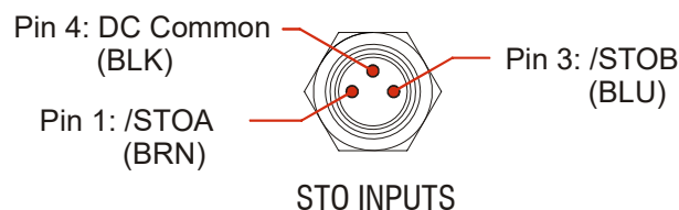
Figure R1.7 STO Connector Pinout
